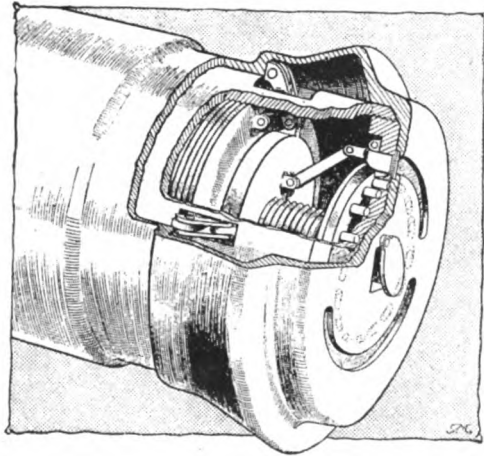
Fig. 4—Perspective sketch showing how the locking toggles project through slots formed in the inner or fixed hub. Also shown are the celluloid covered ports in the end of the detachable hub through which the safety indicator can be seen when the wheel is locked
